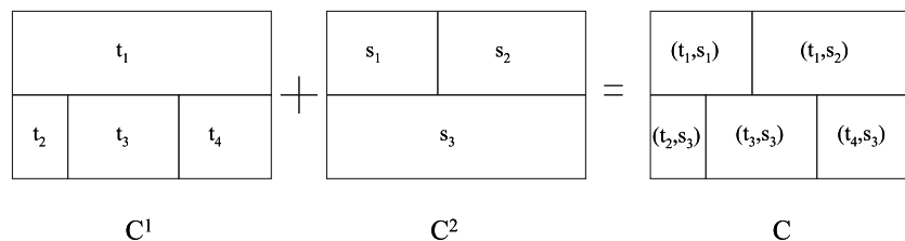
FIG. 7. An example of aggregating two community structure solutions. t_1, t_2, t_3, and t_4 are labels on the nodes in a network obtained from solution 1 and denoted as C^1 . The network is partitioned into groups of nodes having the same labels. s_1, s_2, and s_3 are labels on the nodes in the same network obtained from solution 2 and denoted as C^2 . All nodes that had label t_1 in solution 1 are split into two groups with each group having labels s_1 and s_2 , respectively, while all nodes with labels t_3, t_4, or t_5 in solution 1 have labels s_3 in solution 2. C represents the new labels defined from C^1 and C^2 .
